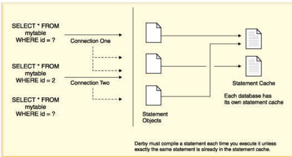
Figure 2. A database can reuse a statement execution plan when the SQL text matches a prior statement exactly ( PreparedStatement s are much more efficient.)
